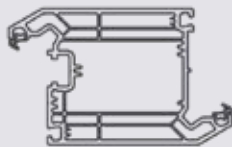
103366 115mm Open In Door Sash/Z Midrail
